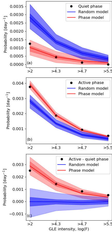
Figure 5. GLE occurrence probability with increasing intensity threshold (a) in the quiet phase, (b) in the active phase, and (c) the difference between the active and quiet phases. Black circles show the observations. The blue lines, dark shaded and light-shaded areas show the median, one-sigma (i.e. 68%) and two-sigma (i.e. 95%) of 5000 Monte Carlo samplings of the Random model, wherein GLEs are assumed to have equal occurrence probability at all times. The red lines and shaded areas show the same for the Phase model, wherein GLEs are a factor four more probable in the active phase than in the quiet phase.
