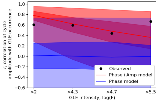
Figure 6. The linear correlation, r_L , between solar cycle amplitude (as measured by the cycle-average sunspot number) and average GLE occurrence probability. Observations are shown by black circles. The blue lines, dark- and light-blue shaded areas show the median, one-sigma (i.e. 68%) and two-sigma (i.e. 95%) of 5000 Monte Carlo samplings of the Phase model, wherein GLEs are assumed to have equal occurrence probability in all cycles. The red lines and shaded areas show the same for the Phase+Amp model, wherein GLE occurrence probability increases linearly with cycle amplitude.
