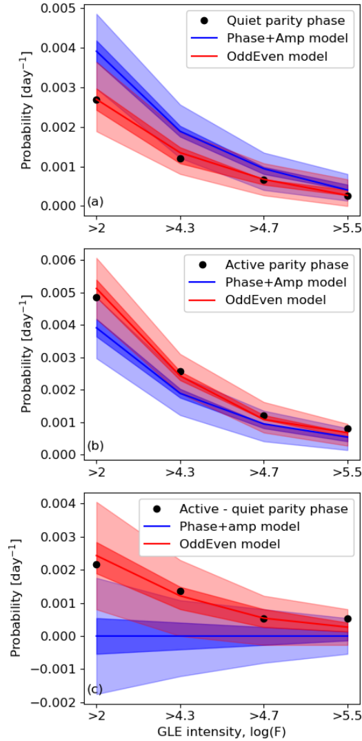
Figure 7. GLE occurrence probability with increasing intensity threshold (a) in the quiet parity phases, i.e. early in even cycles, late in odd cycles, (b) in the active parity phases, i.e. late in even cycles, early in odd cycles, and (c) the difference between the active and quiet parity phases. Observations are shown in black. The blue line, dark shaded and light-shaded areas show the median, one-sigma (i.e. 68%) and two-sigma (i.e. 95%) of 5000 Monte Carlo samplings of the Phase+Amp model, wherein GLEs are assumed to have equal occurrence probability in the early and late active period. The red lines and shaded areas show the same for the OddEven model, wherein GLEs are a factor more probable in the early active phase in even cycles and in the late active phase in odd cycles.
