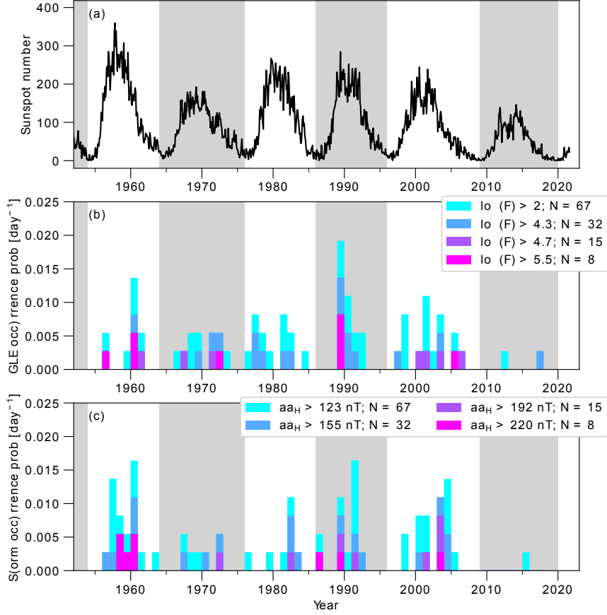
Figure 1. Time series of (a) sunspot number, (b) GLE occurrence and (c) geomagnetic storm occurrence, as determined from the aa_H dataset. White/grey shaded regions show odd/even solar cycles, respectively.
