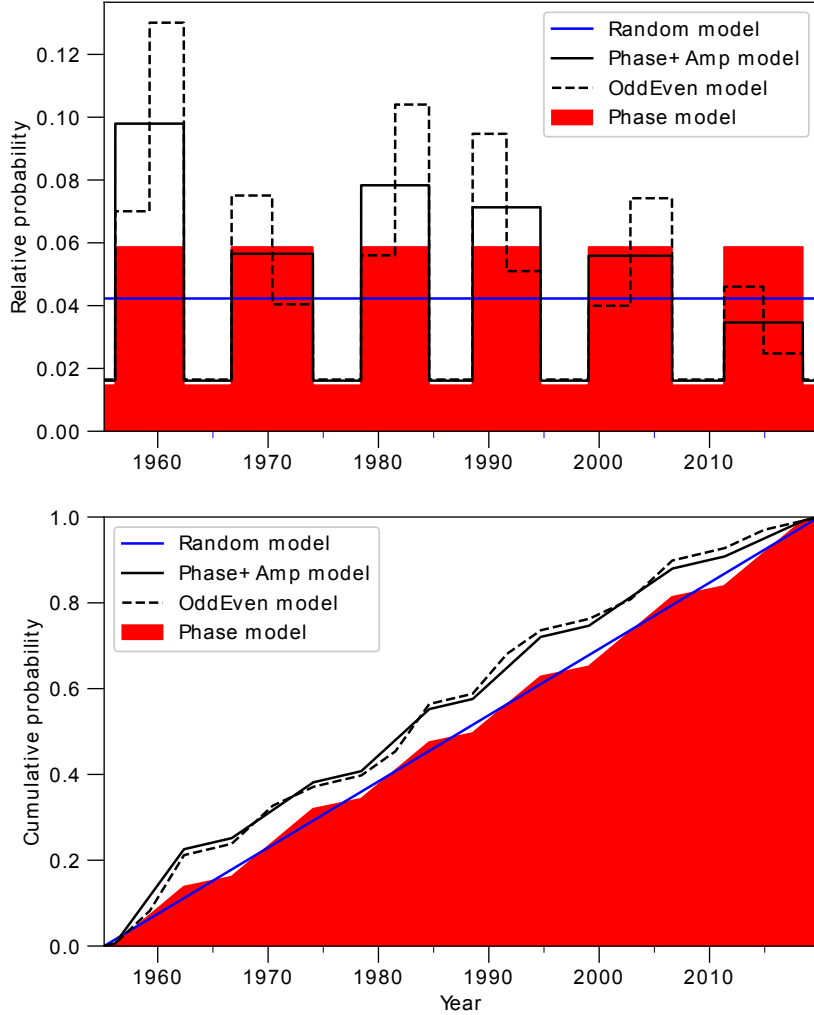
Figure 4. Top: Models of GLE occurrence probability used to make inferences about the observations. Bottom: Cumulative distribution functions of the model probability, from which events are drawn. The Random model (blue) has a constant probability of a GLE at all times. The Phase model (red) has a factor four higher GLE probability during the active phase that the quiet phase. The Phase+ Amp model further weights the active phase by the solar cycle amplitude (taken to be the cycle-average sunspot number). Finally, the OddEven model further adjusts the GLE occurrence probability up or down by a factor 0.3 during the early and late active phases based on the solar cycle parity (i.e. odd or even numbered).
