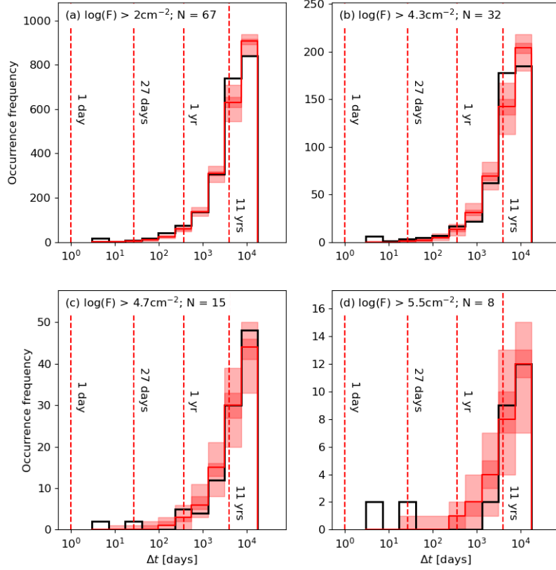
Figure 9. Histograms of the separation times, \Delta t , between all possible GLE pairs for events defined by four different intensity thresholds. Note that the bins are equally spaced in log space. Red dashed vertical lines show a number of times of interest, for reference. Observations are shown in black. The red line, dark shaded and light-shaded areas show the median, one-sigma (i.e. 68%) and two-sigma (i.e. 95%) of Monte Carlo samples of the Random model.
