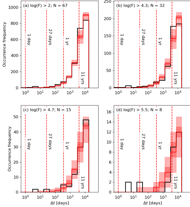
Figure 8. Histograms of GLE waiting times for events defined by four different intensity thresholds. Note that the bins are equally spaced in log space. Red dashed vertical lines show a number of times of interest, for reference. Observations are shown in black. The red line, dark shaded and light-shaded areas show the median, one-sigma (i.e. 68%) and two-sigma (i.e. 95%) of Monte Carlo samples of the Random model.
